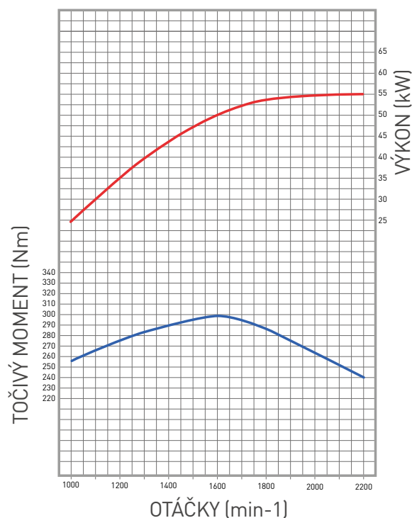
MOTOR TCD 2.9 L4
